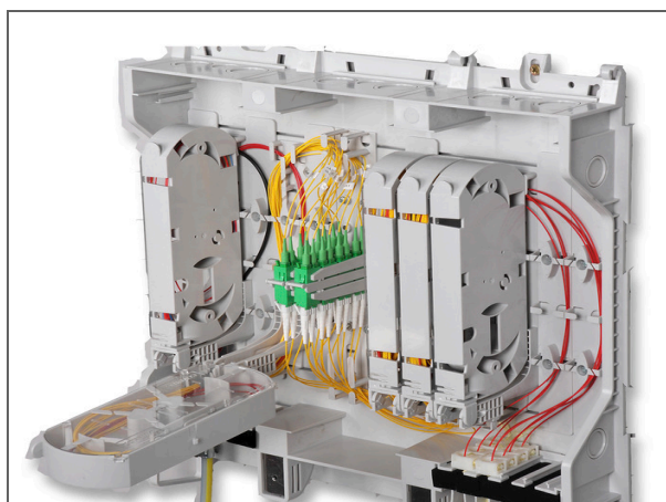
Building Access Terminal (BAT), Size L, gray, EMKA lock, 16 cable strain reliefs
